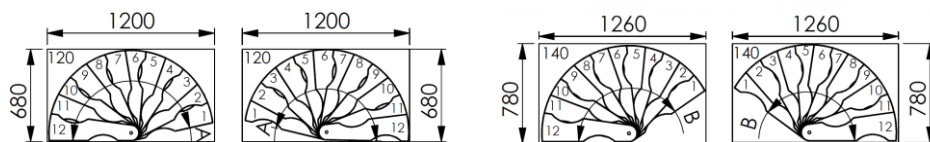
Montagevarianten / Assembling variations
